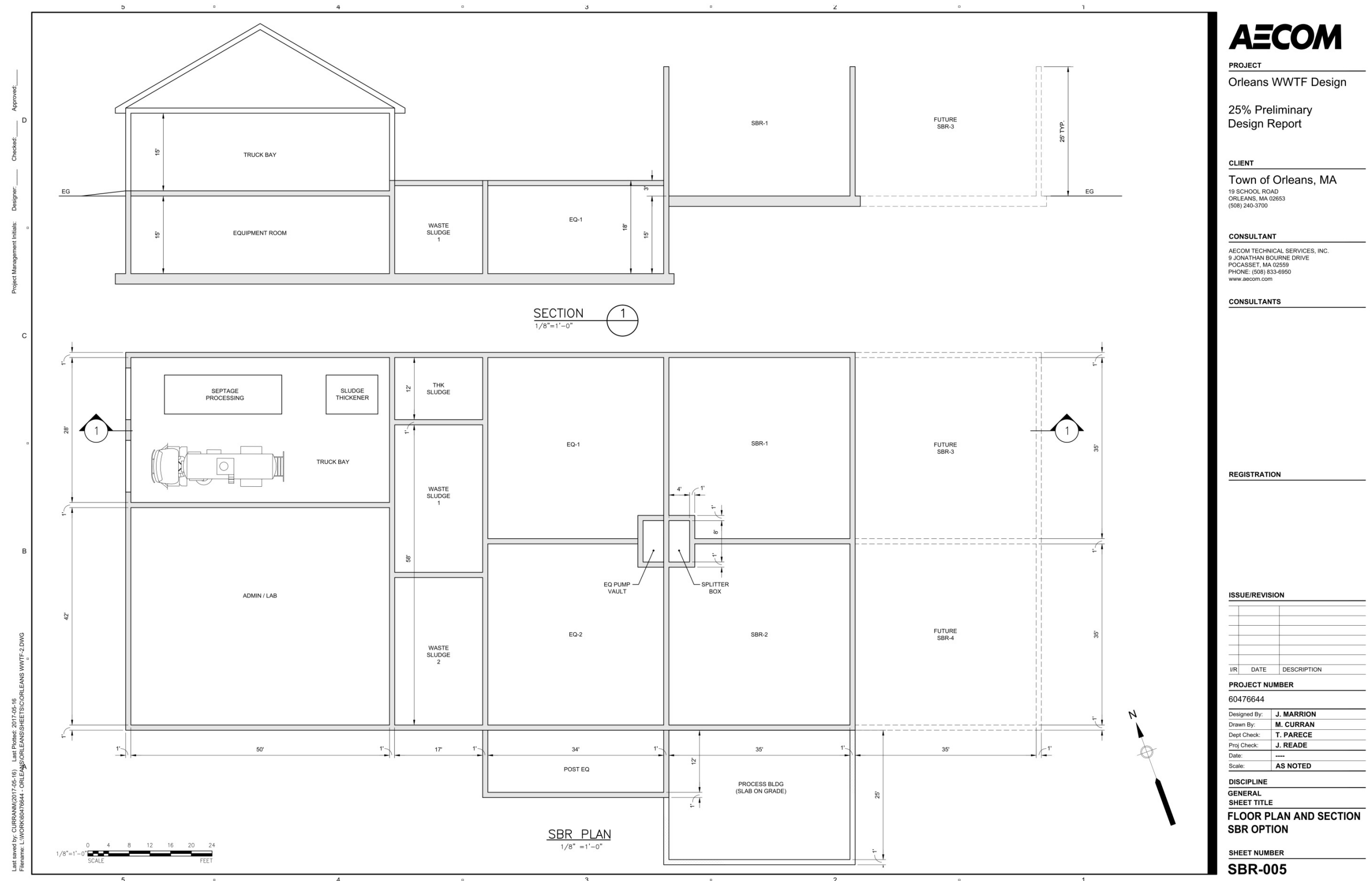
Figure 16: Floor Plan & Section – SBR Option
